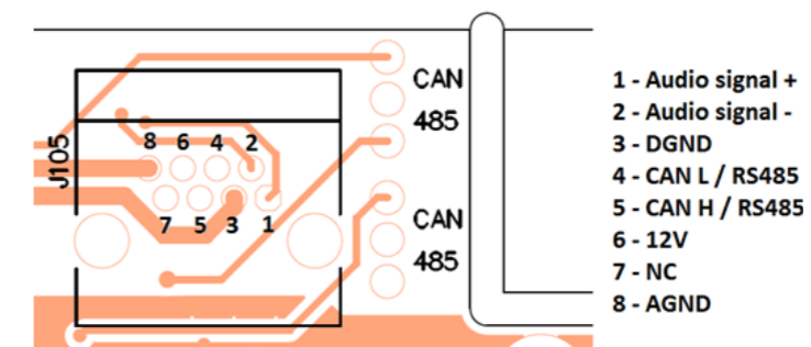
EMAGPE16RJ45 connector pinout diagram CAN bus mode
