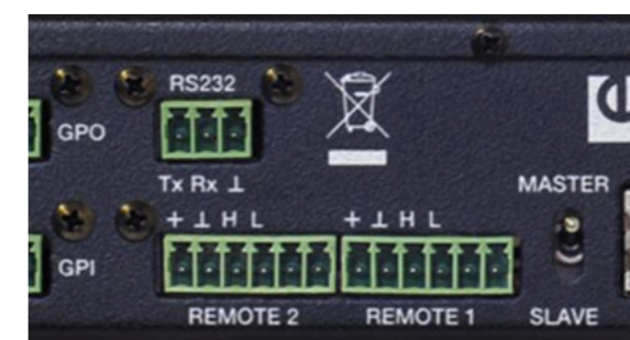
REMOTE ports in the back panel of PXN matrices
