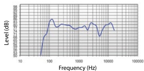
Frequency response
