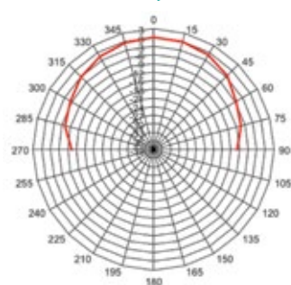
Directivity @ 1kHz
