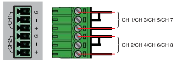
[Unbalanced cable]
