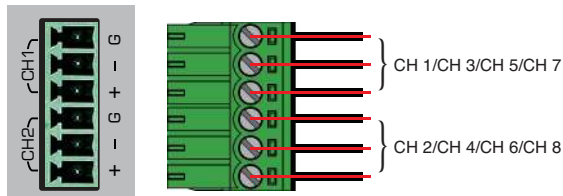
[Balanced cable]
