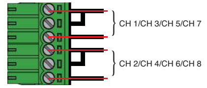
[Unbalanced cable]
