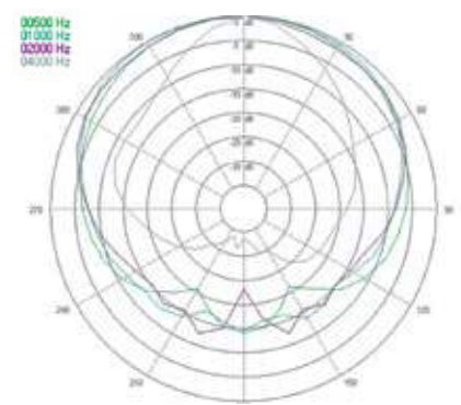
Directivity
