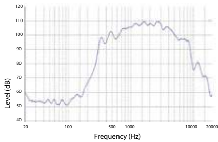
Bandwidth
