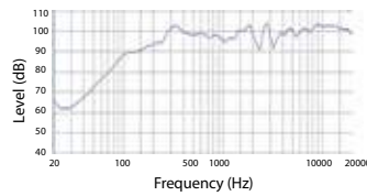
Bandwidth
