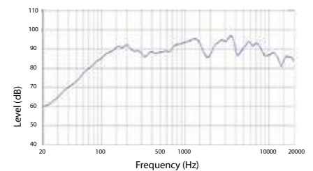
Bandwidth
