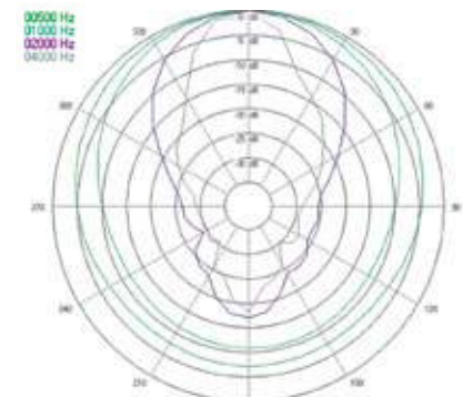
Bandwidth
