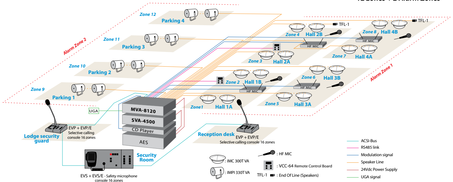
Example of sound security system, 12 zones + 2 Alarm Zones
