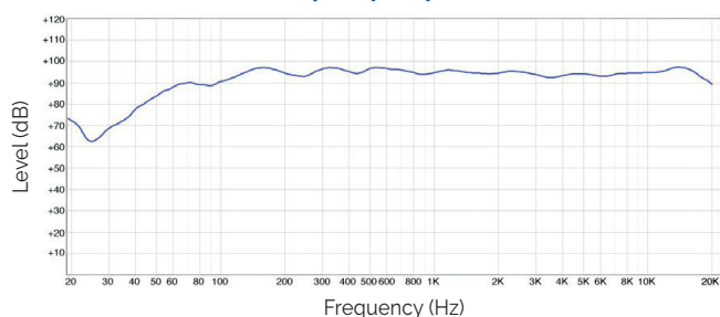
Frequency Response
