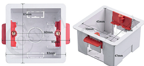
BOITIER PM E : Wall mounting box (optional)
