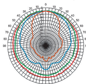
Horizontal directivity
