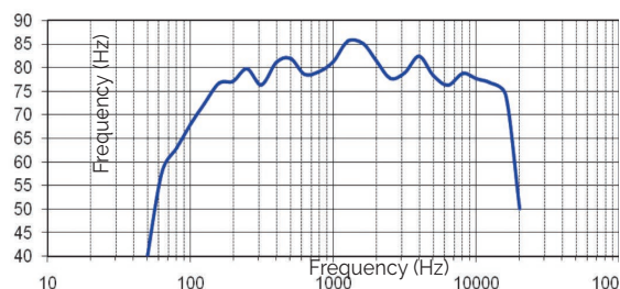
Bandwidth
