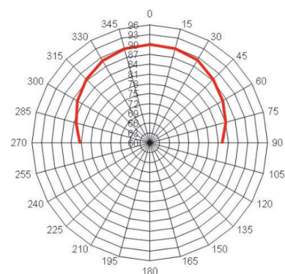
Directivity @ 1kHz
