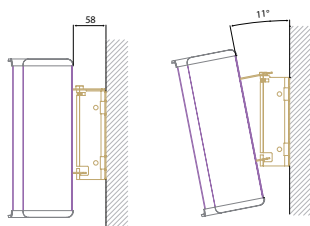
Vertical maximum 11°
