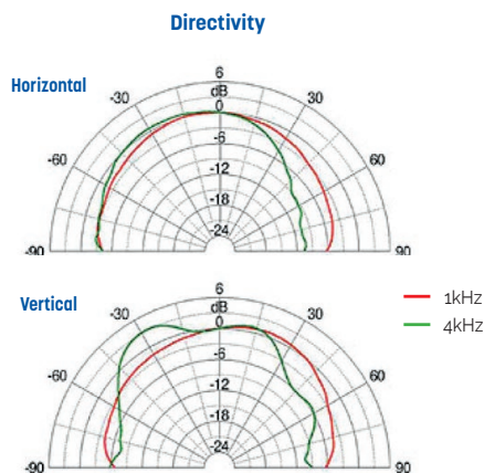
Directivity
