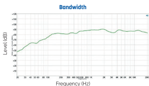
Bandwidth
