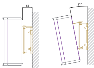
Fixing Bracket Vertical maximum 11°
