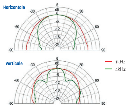
Directivity
