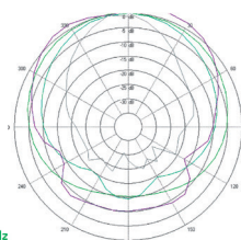
Horizontal directivity
