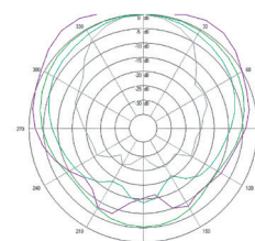
Vertical directivity
