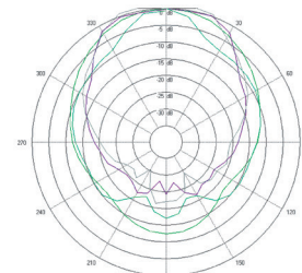
Vertical directivity
