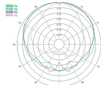
Directivity
