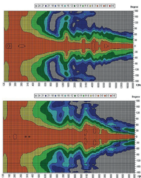
Polar diagrams
