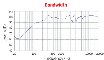
Horizontal directivity
