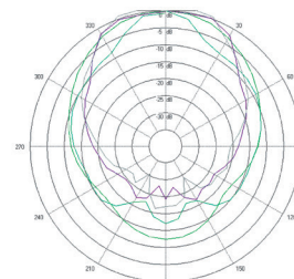
Vertical directivity
