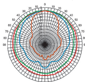
Horizontal directivity
