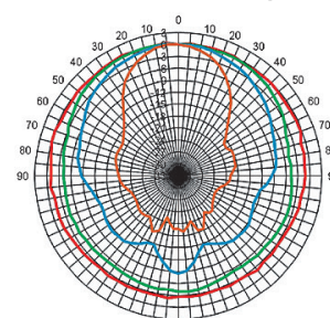
Vertical directivity
