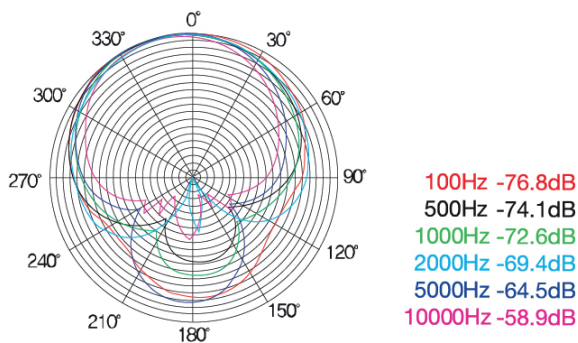
Polar pattern
