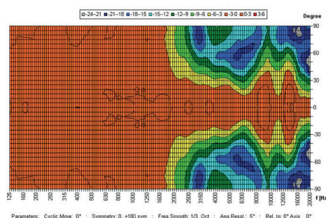
Polar diagrams
