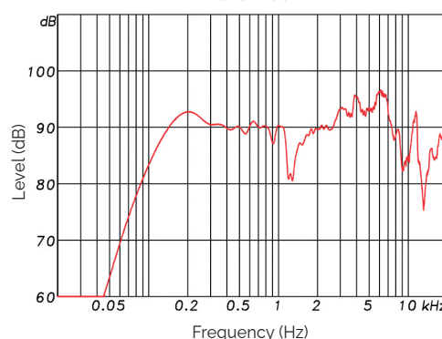
Bandwidth
