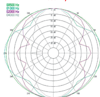
Directivity
